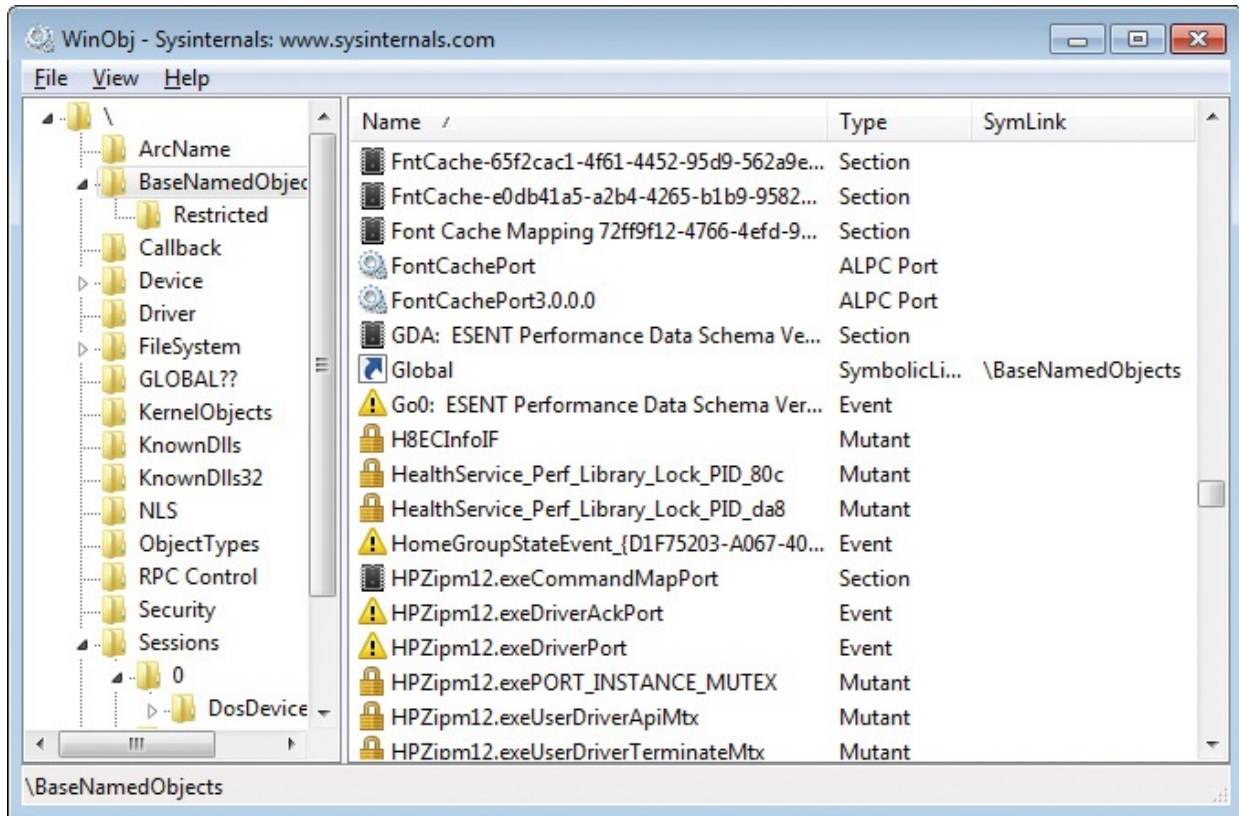
FIGURE 15-12 WinObj.
