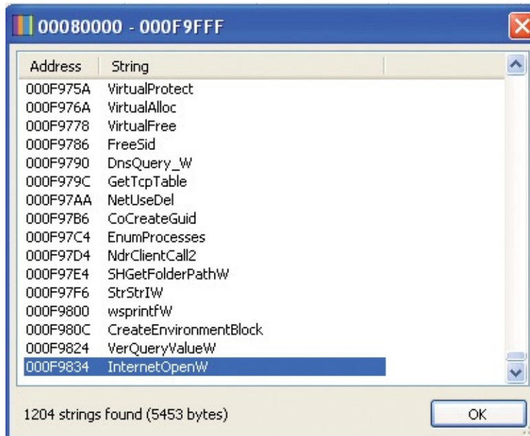
FIGURE 20-9 Text from the injected DLL’s import table.
