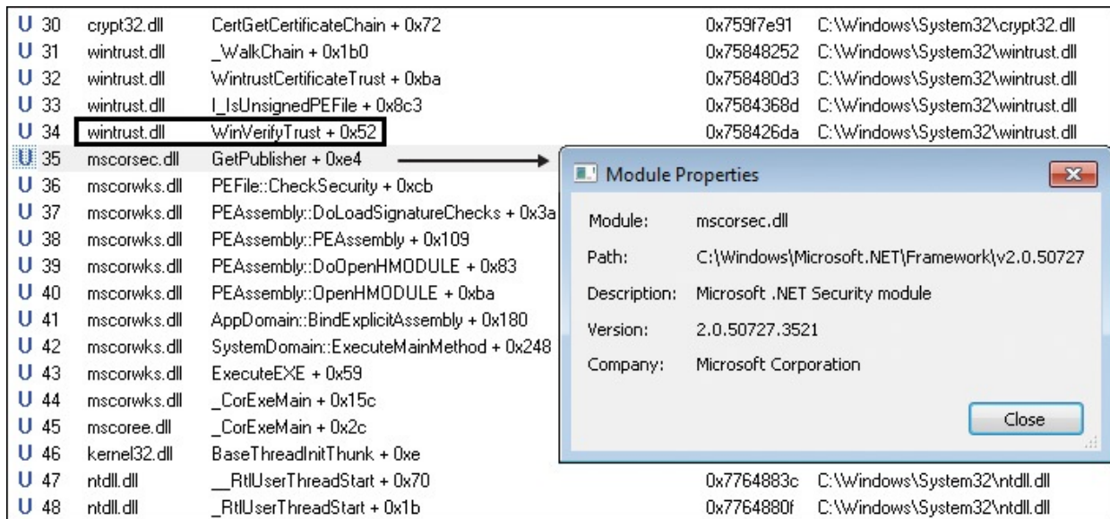
FIGURE 19-40 .NET Framework invoking WinVerifyTrust .
