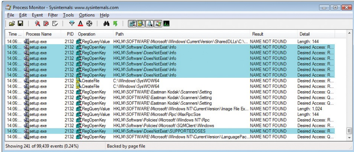
FIGURE 17-20 Highlighting “DoesNotExist” in the filtered results.
