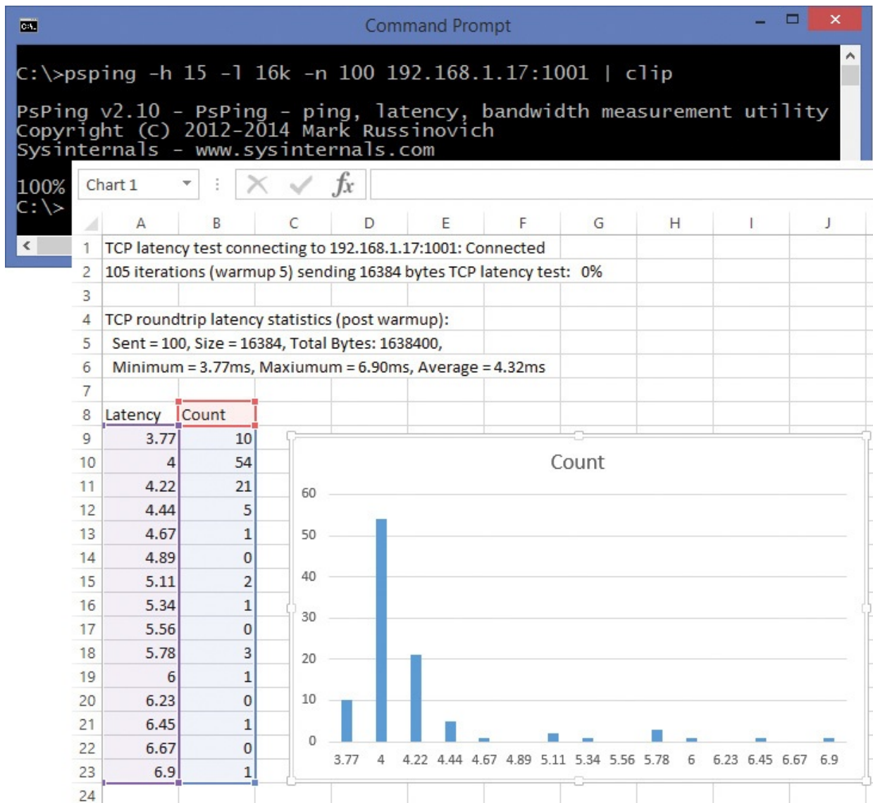
FIGURE 14-7 Copying PsPing histogram data to the clipboard and creating a chart with it in Microsoft Excel.
