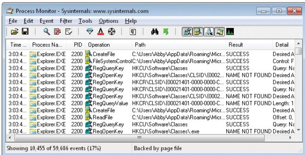
FIGURE 5-1 Process Monitor.
