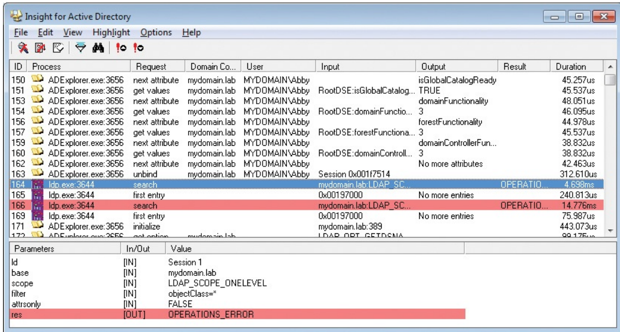
FIGURE 10-10 AdInsight.
