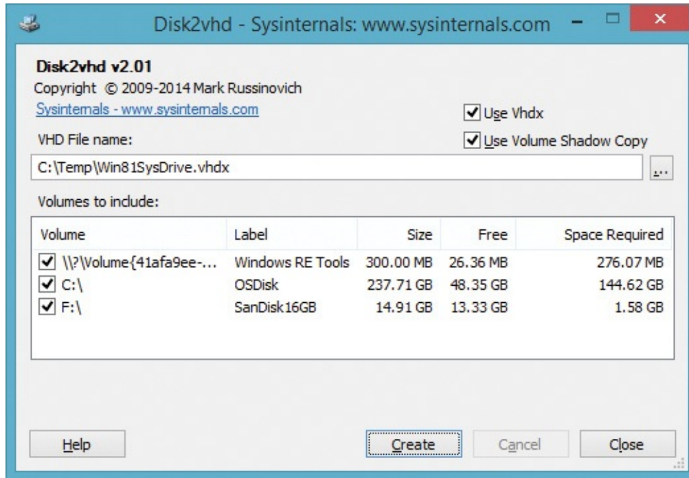
FIGURE 13-1 Disk2Vhd.
