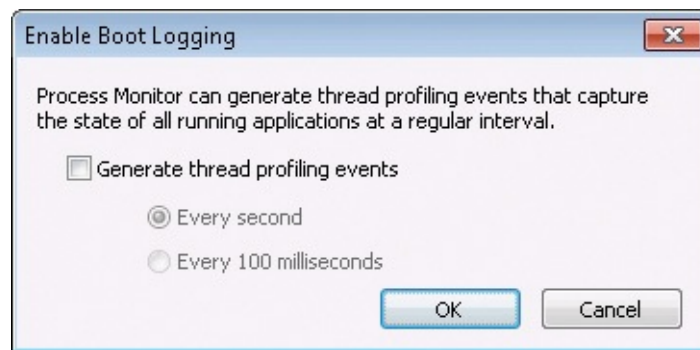
FIGURE 5-20 Boot-logging options
