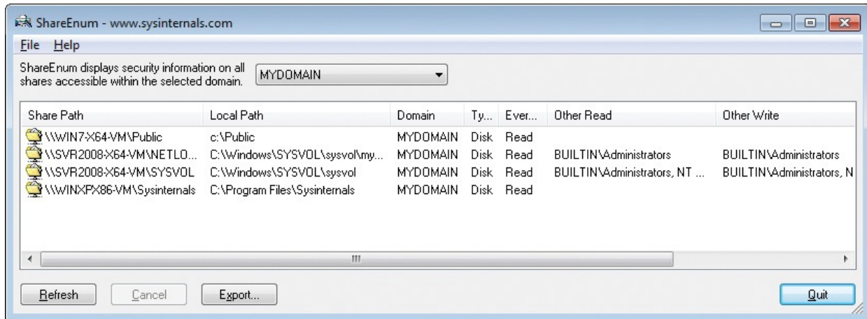
FIGURE 9-10 ShareEnum.
