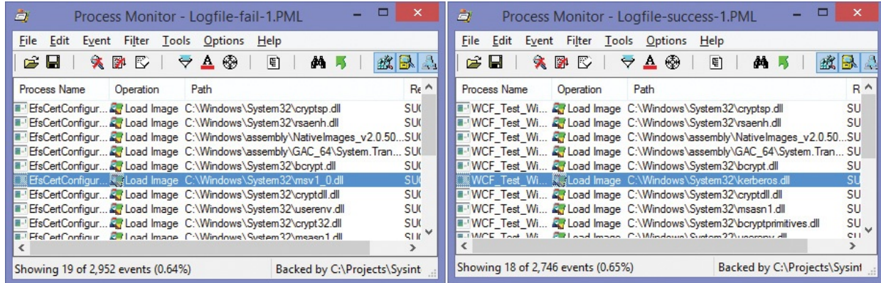
FIGURE 22-1 The failing trace loads Msv1_0.dll, while the working version loads Kerberos.dll.
