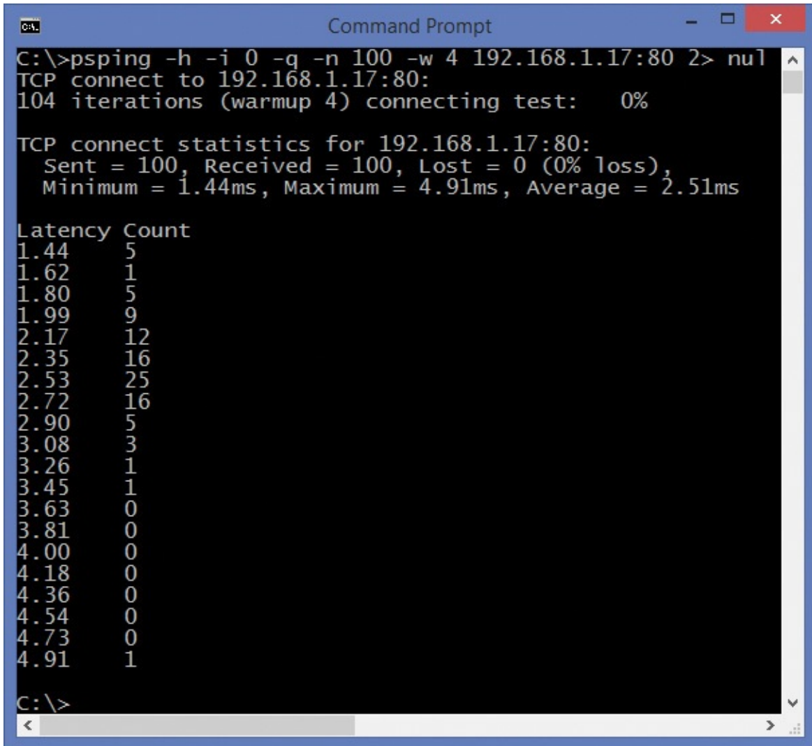
FIGURE 14-6 PsPing default histogram.
