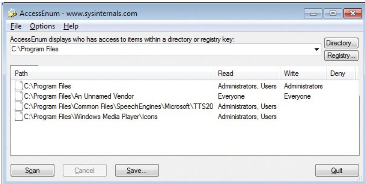
FIGURE 9-9 AccessEnum.
