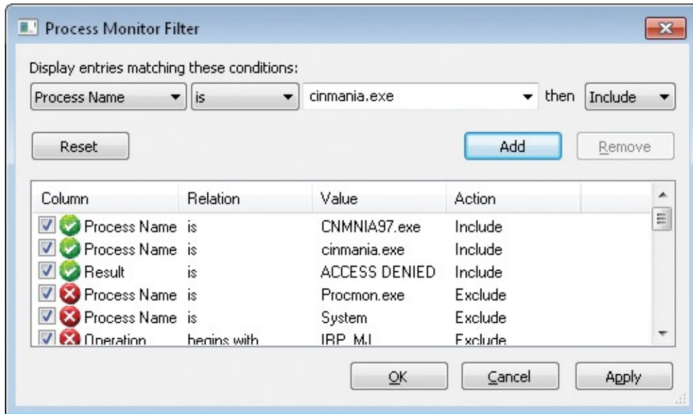
FIGURE 5-11 Process Monitor Filter dialog box.
