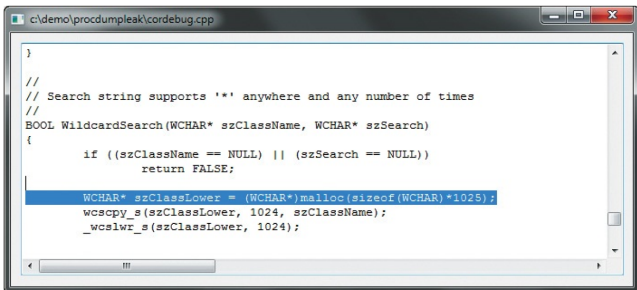
FIGURE 22-11 The line of source code that performed the heap allocation
