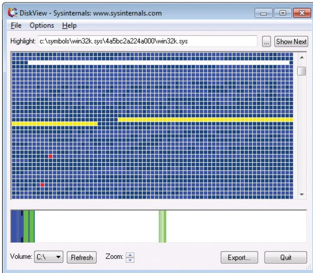
FIGURE 13-15 DiskView.
