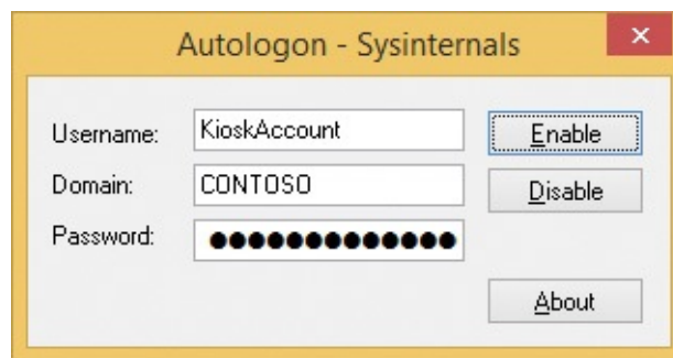
FIGURE 9-13 Autologon.
