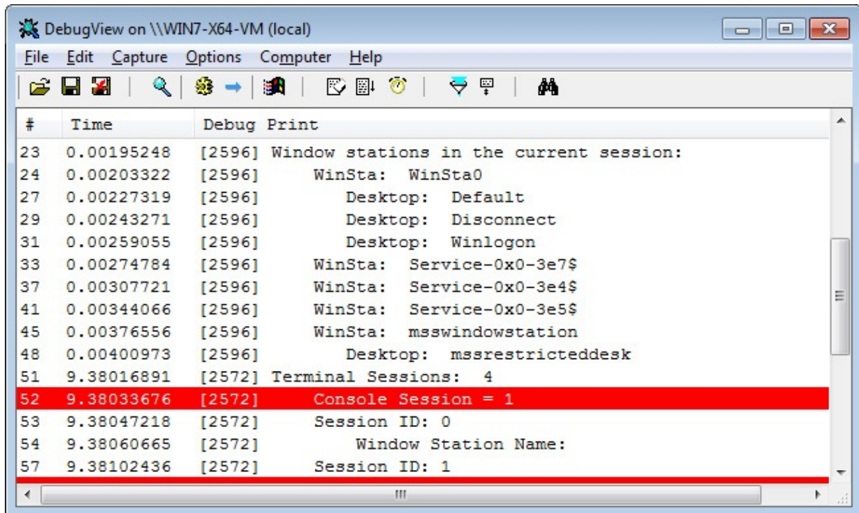
FIGURE 8-13 DebugView.
